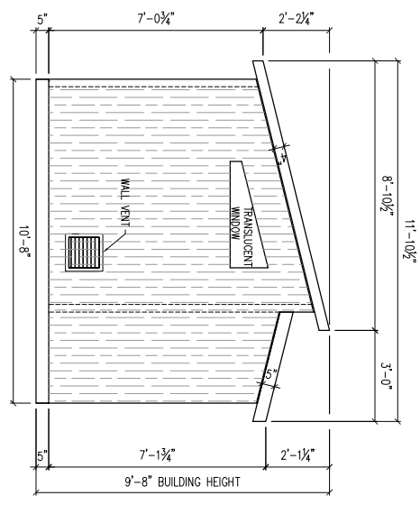
LEFT ELEVATION
