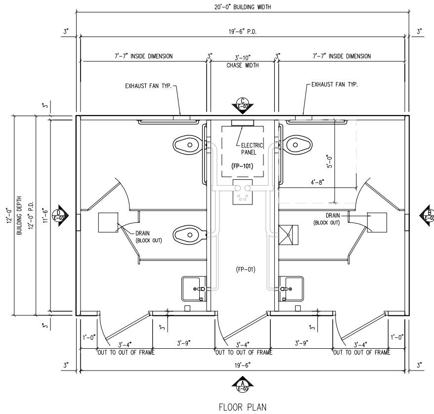
FLOOR PLAN
