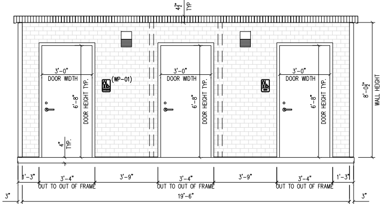
A FRONT ELEVATION E-03
