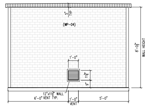
D LEFT ELEVATION E-03
