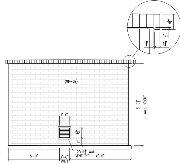
B RIGHT ELEVATION E-03
