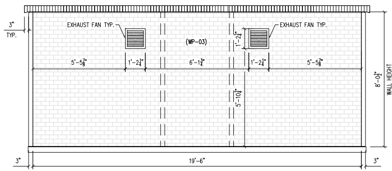
C REAR ELEVATION E-03
