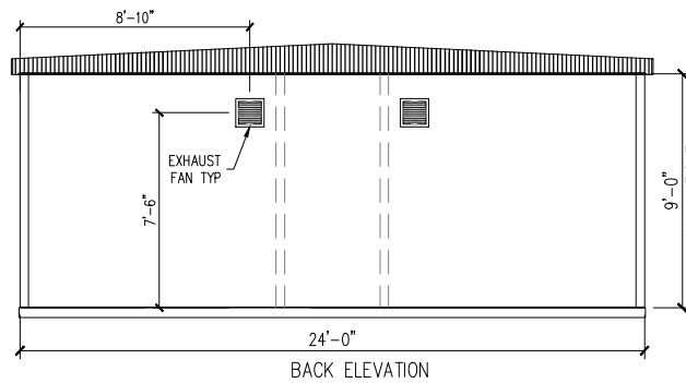
BACK ELEVATION
