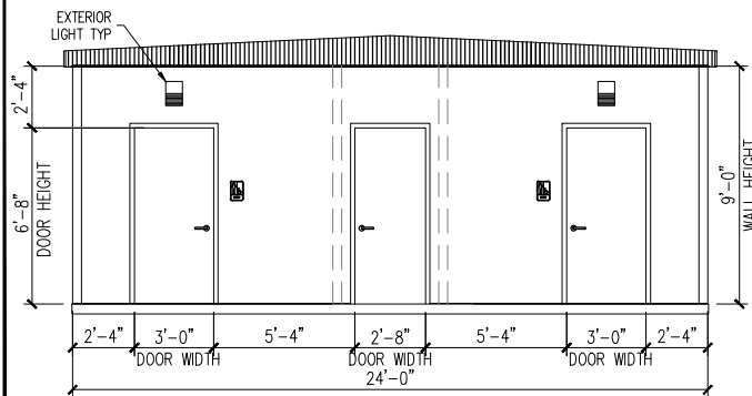
BUILDING LAYOUT FRONT ELEVATION
